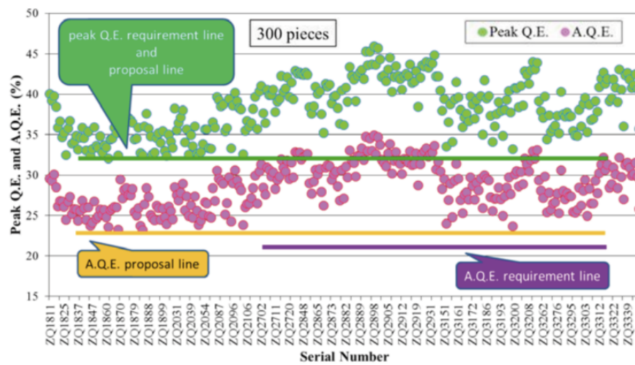
Figure 4. Peak QE of 300 PMTs produced by Hamamatsu in 2013 (green circles). The QE curve fold with the Cherenkov spectrum from 100 GeV gamma showers (pink circles) shows the average over the Cherenkov spectrum \langle QE_{ch} \rangle . The green and the yellow horizontal lines show the requested in the past minimum values for the peak QE and the \langle QE_{ch} \rangle .
