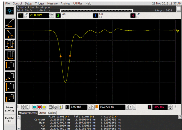
Figure 8. Pulse width of a Hamamatsu 7-dynode PMT operated under 1000 V.
