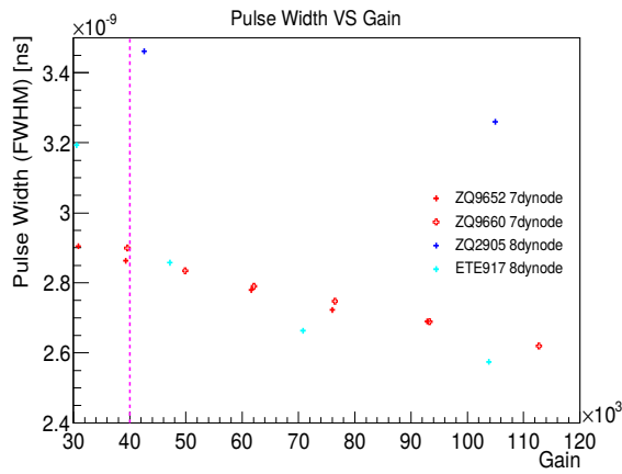
Figure 7. PMT pulse width versus gain (applied HV) for Hamamatsu and ETE PMTs.
