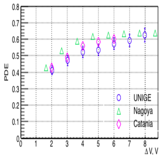
Figure 9. Cross-check of PDE as a function of Overvoltage at 405 nm wavelength, between three partners.
