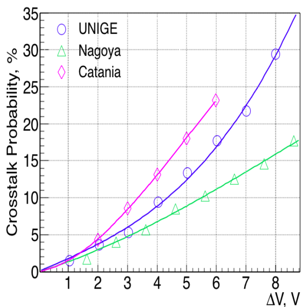
Figure 11. Cross-check of P_{XT} as a function of Overvoltage, between three partners first results.
