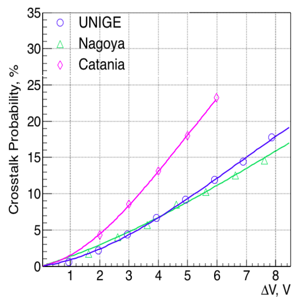
Figure 12. Cross-check of P_{XT} as a function of Overvoltage, between three partners, improved results.
