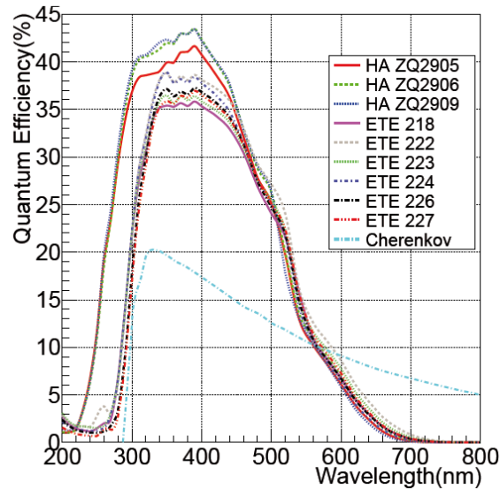
Figure 3. The measured QE of six experimental PMTs from ETE and three PMTs from Hamamatsu. The dashed curve shows the measured on Earth shape of the Cherenkov spectrum, induced by an impinging 100 GeV gamma ray.
