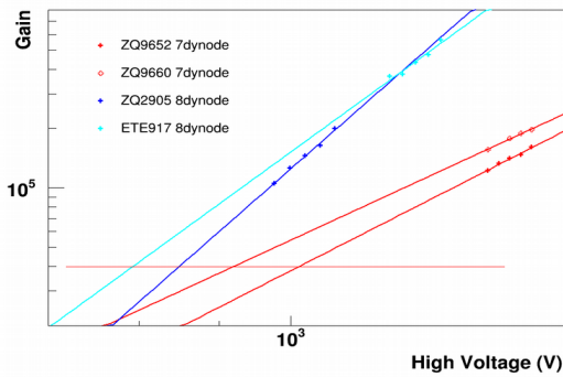
Figure 5. Gain versus applied HV for the Hamamatsu 7-dynode and 8-dynode PMTs.
