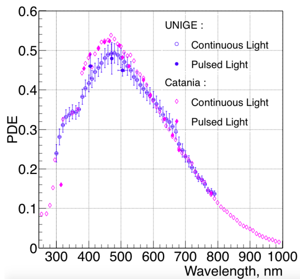
Figure 10. Cross-check of PDE as a function of wavelength at 3 V overvoltage. Results were obtained by University of Geneva and Catania Observatory.
