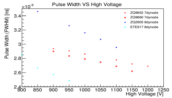
Figure 6. PMT pulse width versus applied HV distribution for Hamamatsu and ETE PMTs.
